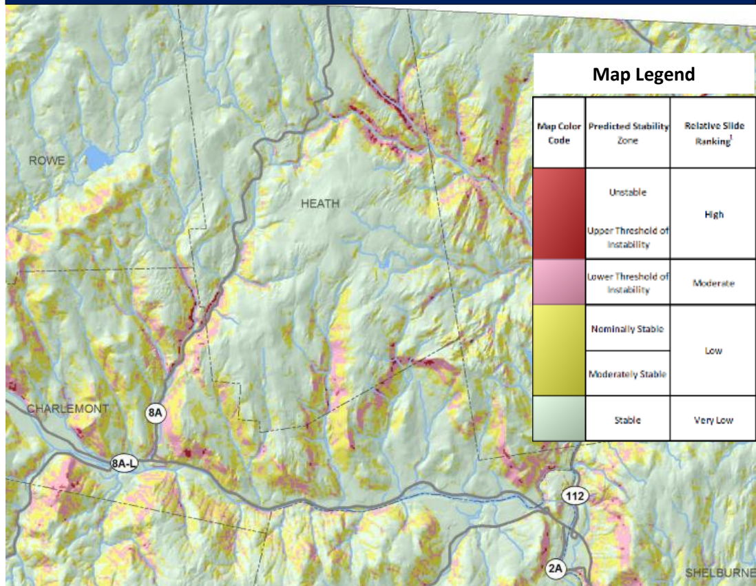
Figure 3-23: Slope Stability Map, Heath and Surrounding Towns
